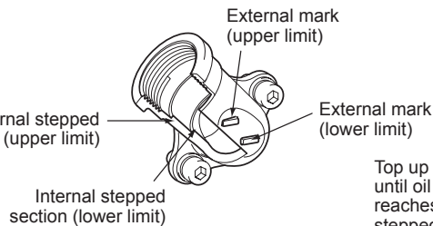
Fig. 2 Oil pipe
